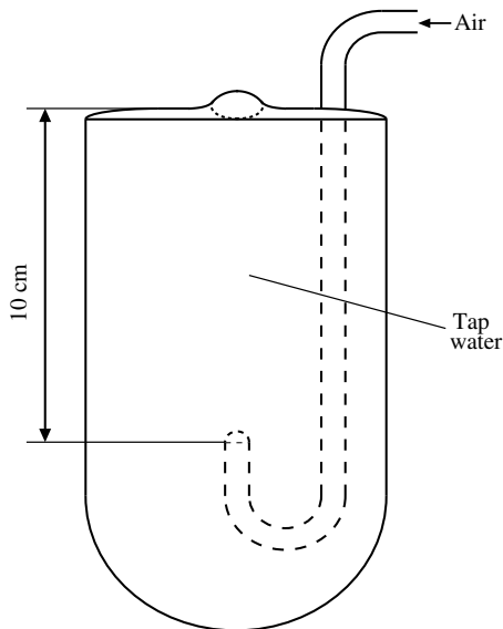
FIGURE 3. Bubbles are generated by injecting pressurized air into a bent pipe. Different bubbles sizes are obtained by changing the pipe outlet diameter and the air flow rate.
