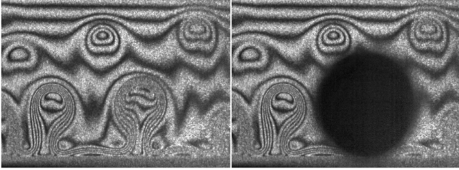
FIGURE 15. Spontaneous bursting at the foot of a flat water film (interference fringes visualized by a monomode argon laser at 488 nm). Nucleation is seen to occur around a convection cell: the paradigm situation in the bursting of bubbles. Image height is 3 mm and time lapse between the two images is 1/3000 s. The film receding velocity is V = 2.8 \text{ m s}^{-1} corresponding to a thickness h = 20 \text{ }\mu\text{m} .
