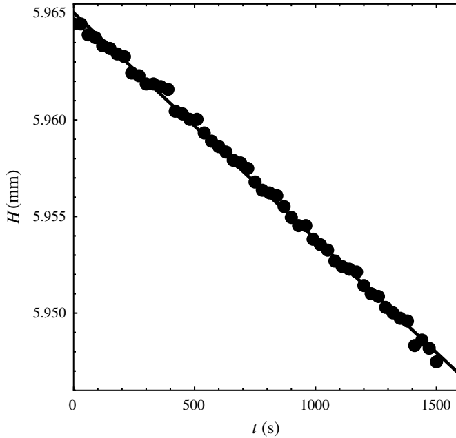
FIGURE 25. Evolution in time of the thickness H of a tapwater layer evaporating in the standard conditions of the laboratory (quiescent air at temperature 20.5^\circ\text{C} , water is thermalized, air hygrometry is 65% of the saturation). The measurement is made by weighting the liquid contained in a circular Petri dish 95 mm in diameter and 12.5 mm deep, with a 1 mg precision balance. The line is the best linear fit giving an evaporation velocity of 11.7 \text{ nm s}^{-1} .
